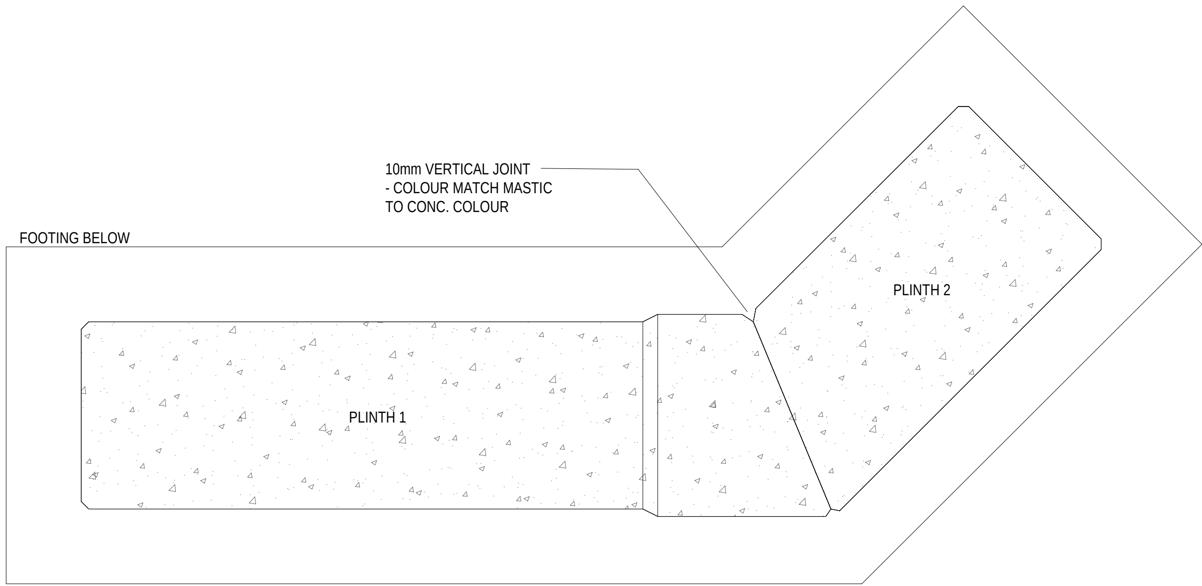
1 WALL TYPE 1 - CONCRETE PLINTH ARRANGEMENT (PLAN) SCALE - 1 : 10
