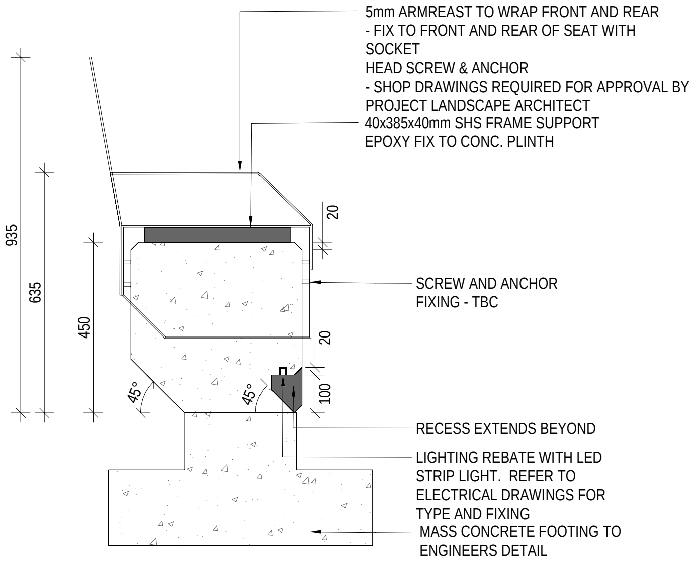
5 WALL TYPE 1 - LED LIGHT REBATE SCALE - 1 : 10
