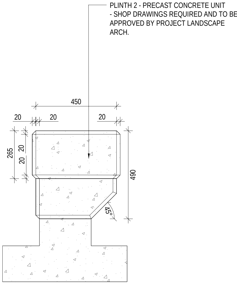
4 WALL TYPE 1 - END ELEVATION SCALE - 1 : 10
