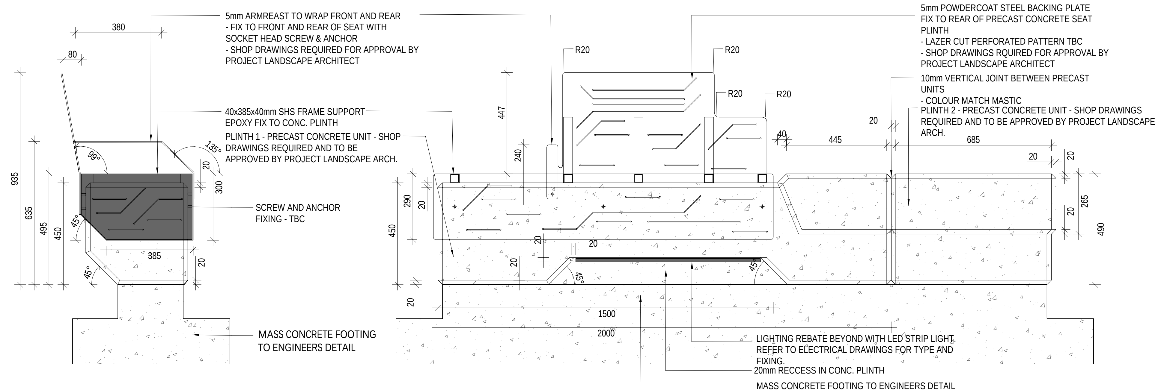
3 WALL TYPE 1 - END & FRONT ELEVATION SCALE - 1 : 10
