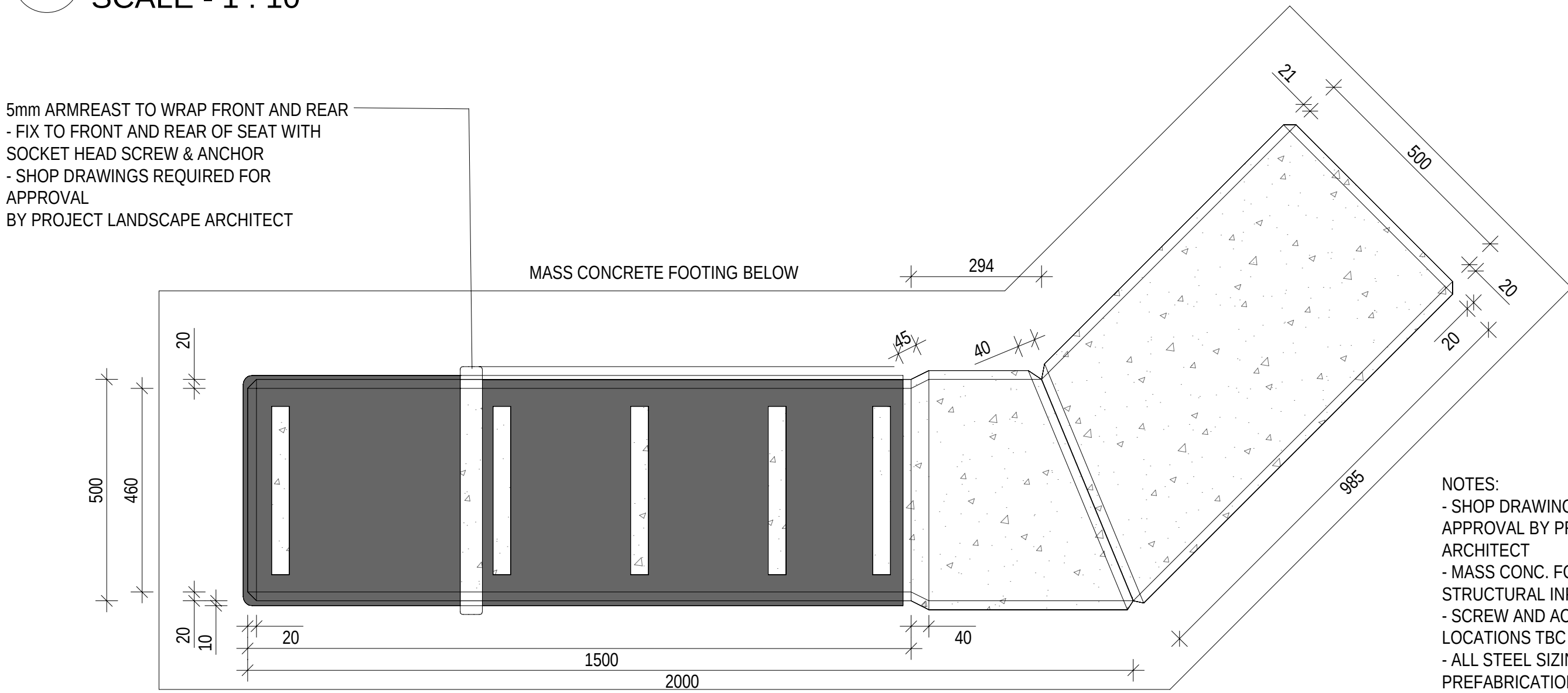
1 WALL TYPE 1 - CONCRETE PLINTH ARRANGEMENT (PLAN) SCALE - 1 : 10
